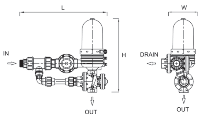
Filter in Filtration mode
